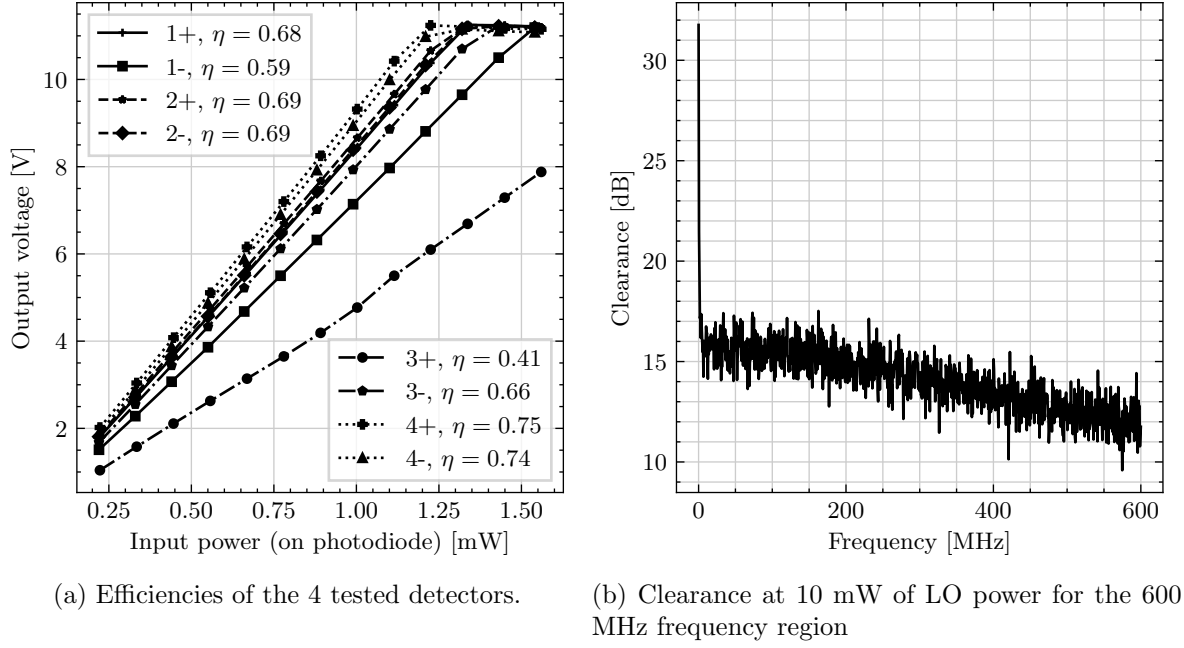
Figure 5.11: Characterisation of the PDB480AC detector.
