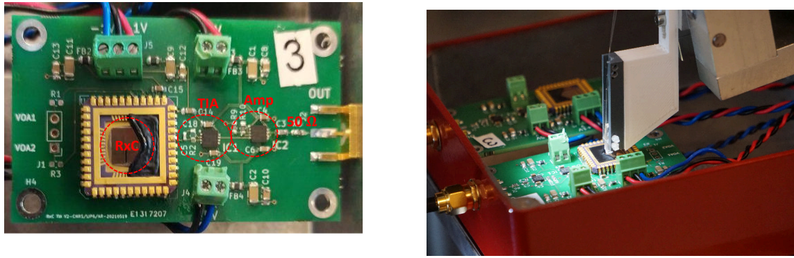
(a) Pictures of the RxC chip in its first electrical package. (b) Coupling mechanism for the early version of the packaged RxC.
