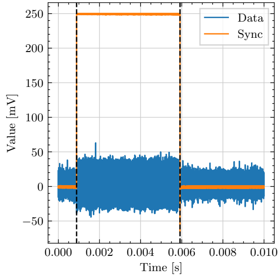
(a) Synchronisation mechanism.
