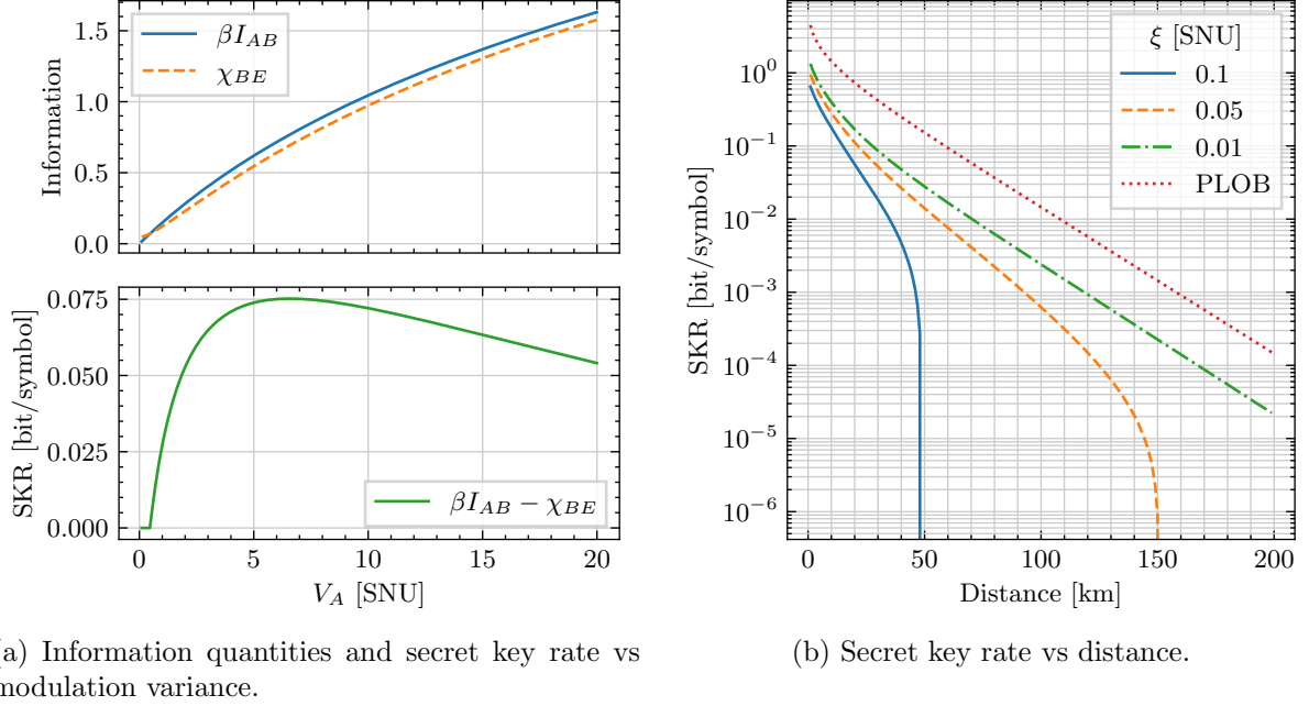
Figure 3.8: CV-QKD asymptotic secret key rate vs modulation variance and distance.
