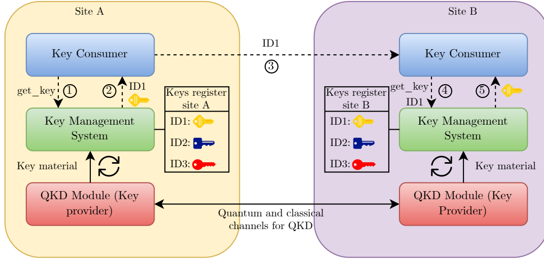
Figure 8.7: Messages order for the ETSI QKD 014 protocol.
