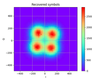
(a) QPSK.
