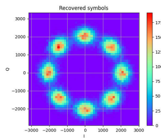
(b) 8-PSK.
