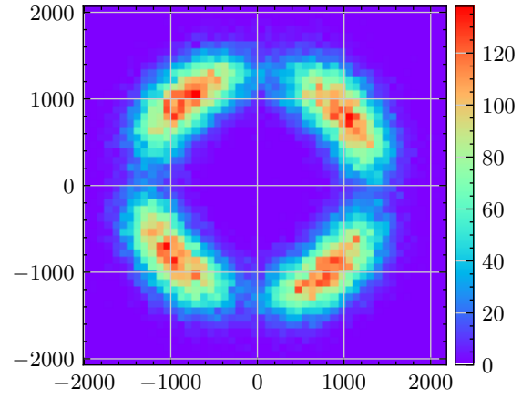
(b) Recovery of a QPSK.
