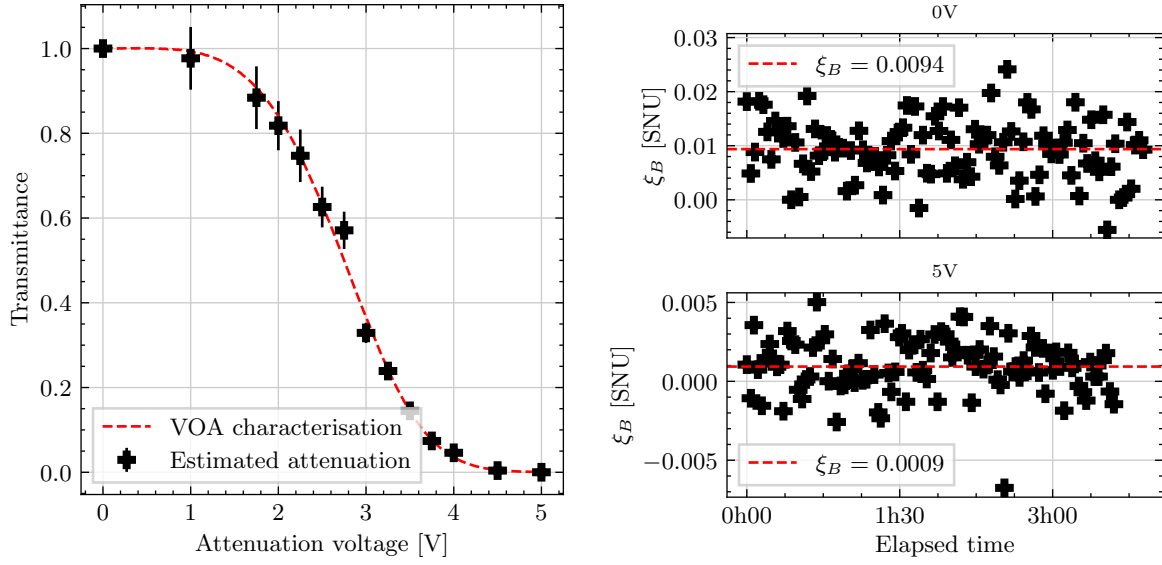
(a) Estimated transmittance vs VOA characterisation.
